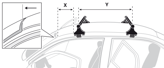
RENAULT Megane, 3-dr Coupé, 97-02
